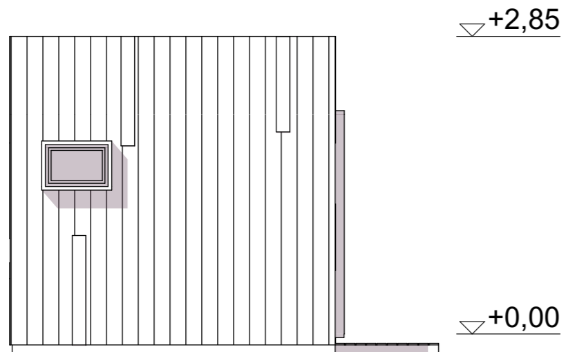
FACADE PIGNON
