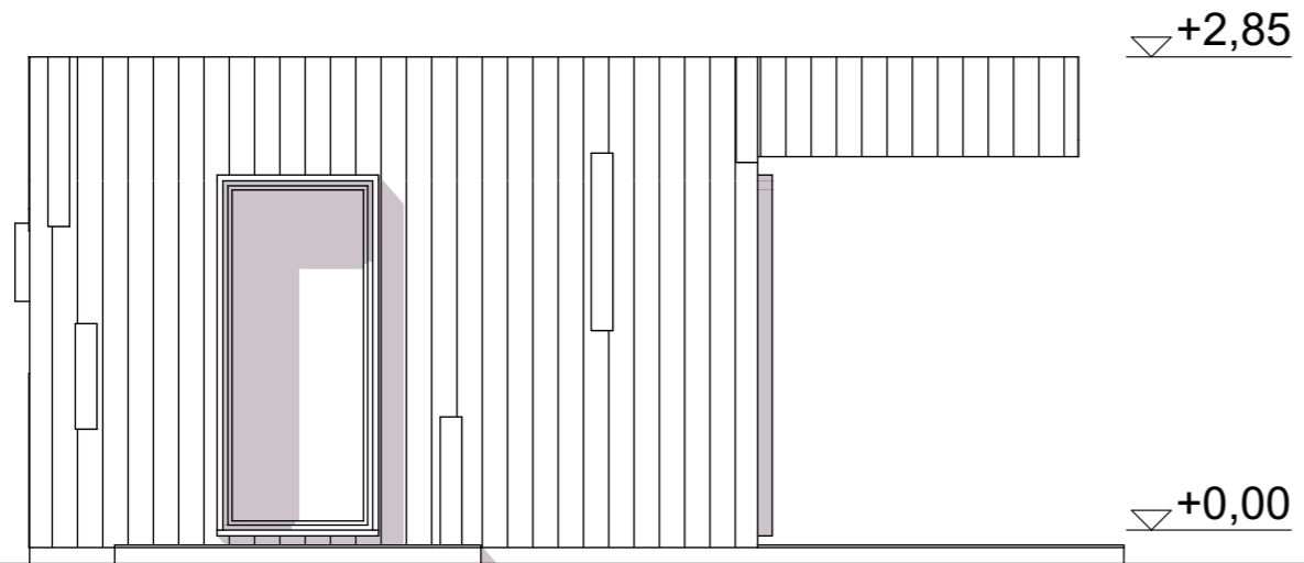
FACADE ENTREE
